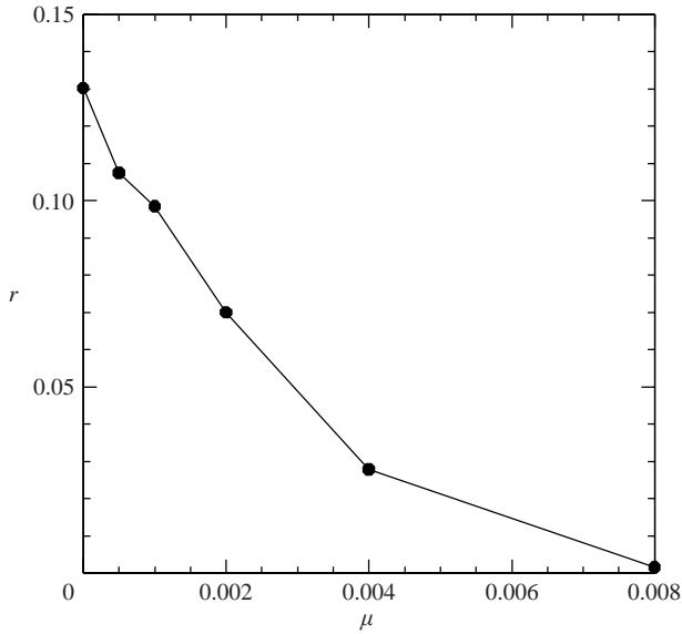
FIGURE 4. The decay of the inverse cascade strength r for the dissipation term -6 \times 10^{-6} \Delta^2 \psi + \mu \Delta \psi as \mu is increased.
