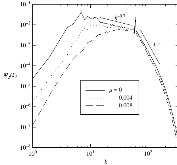
FIGURE 3. The quasi-steady energy spectrum \Psi_2(k) vs. k averaged between t = 15.67 and t = 16.52 for the dissipation term -6 \times 10^{-6} \Delta^2 \psi + \mu \Delta \psi , using three different values of \mu .
